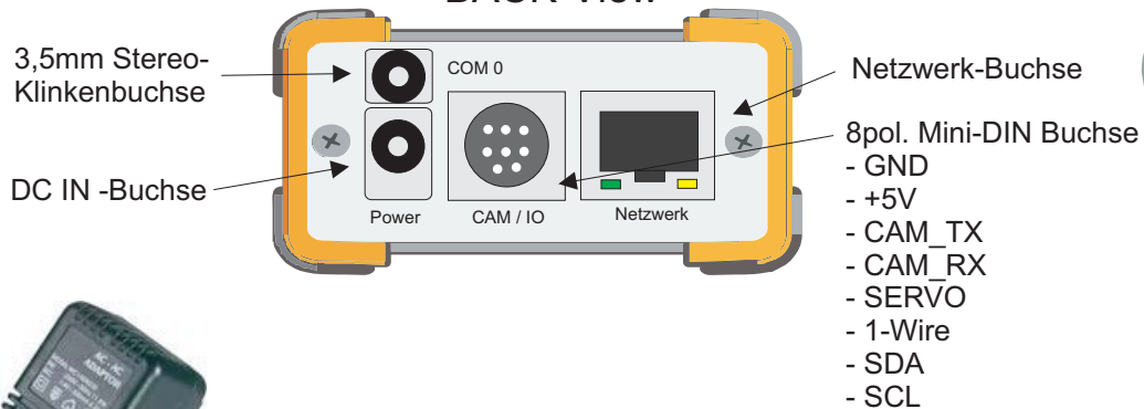
BACK-View
